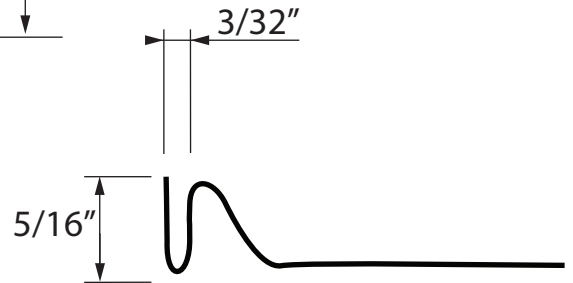
Section View of spin on flange
